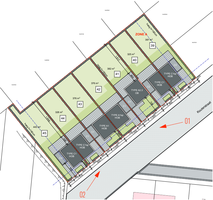
projectzone A 1:500
